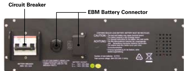
Powerware 9140 EBM (rear view)
