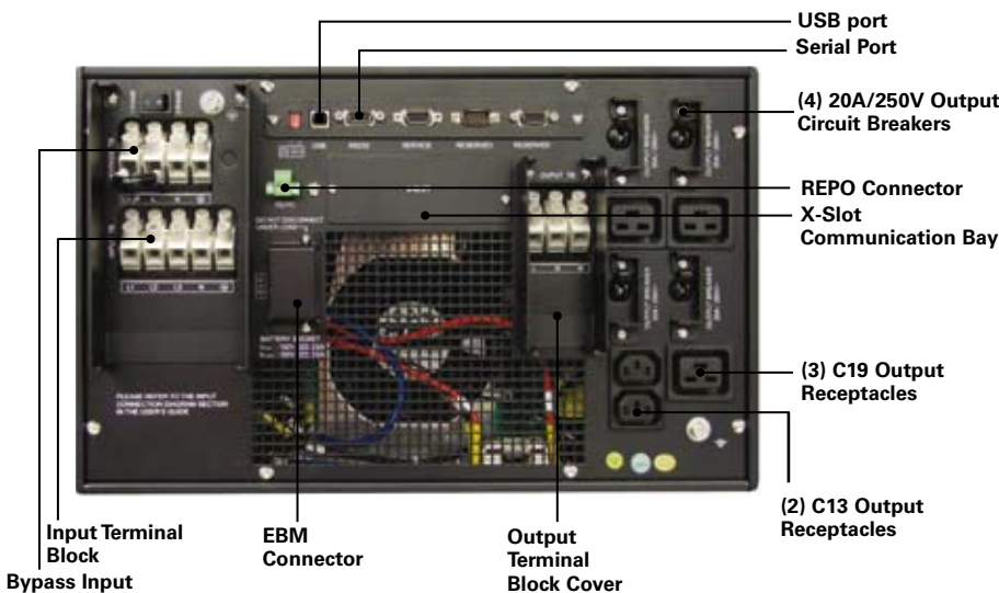
Powerware 9140 (rear view)
